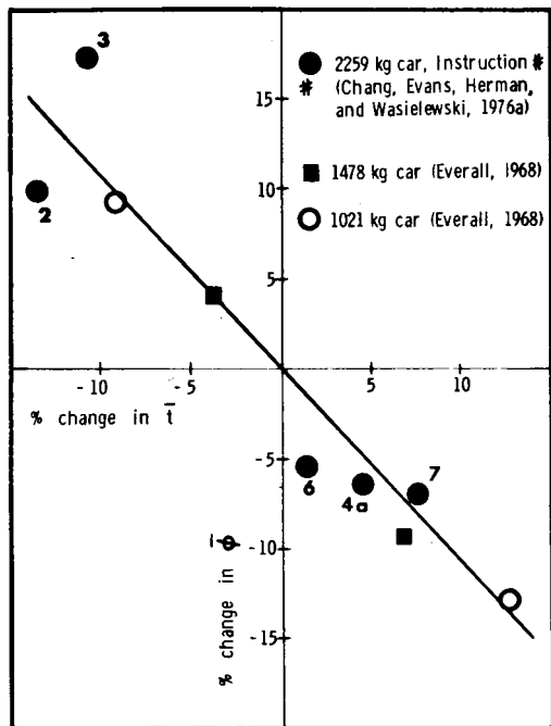
Figure 5. The percentage change in fuel consumption versus the percentage change in trip time for data given in Tables 1 and 2.
